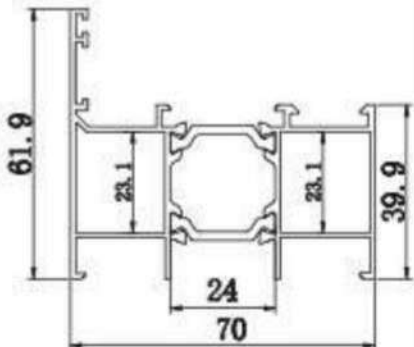
Štok ravan 70 mm
