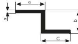
Z - PROFİLLERİ Z - PROFILES / Z - PROFILE
